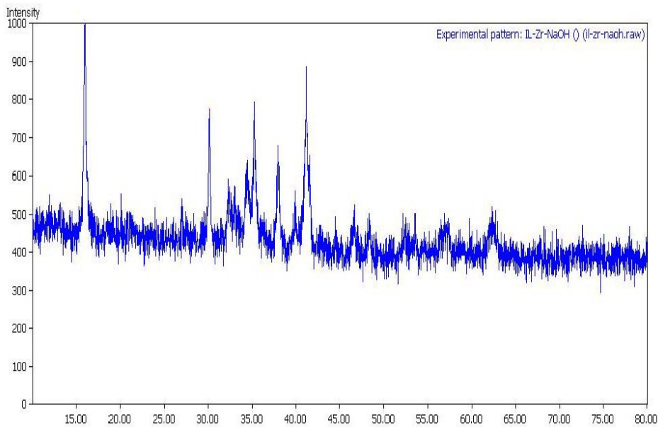
Figure 1. XRD characterization result of the sample at 400^\circ\text{C} .
